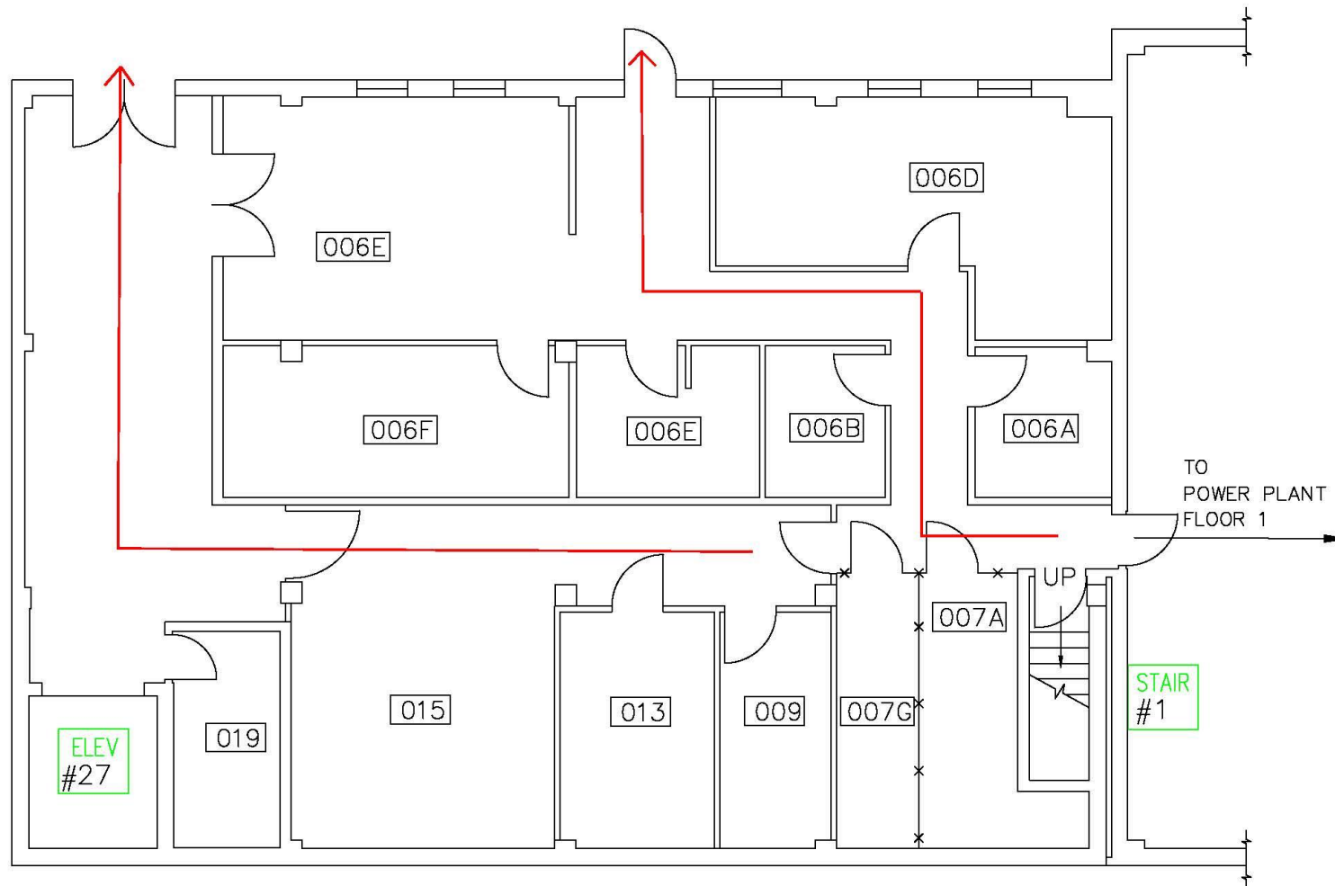
PLANT OPERATIONS GROUND FLOOR
